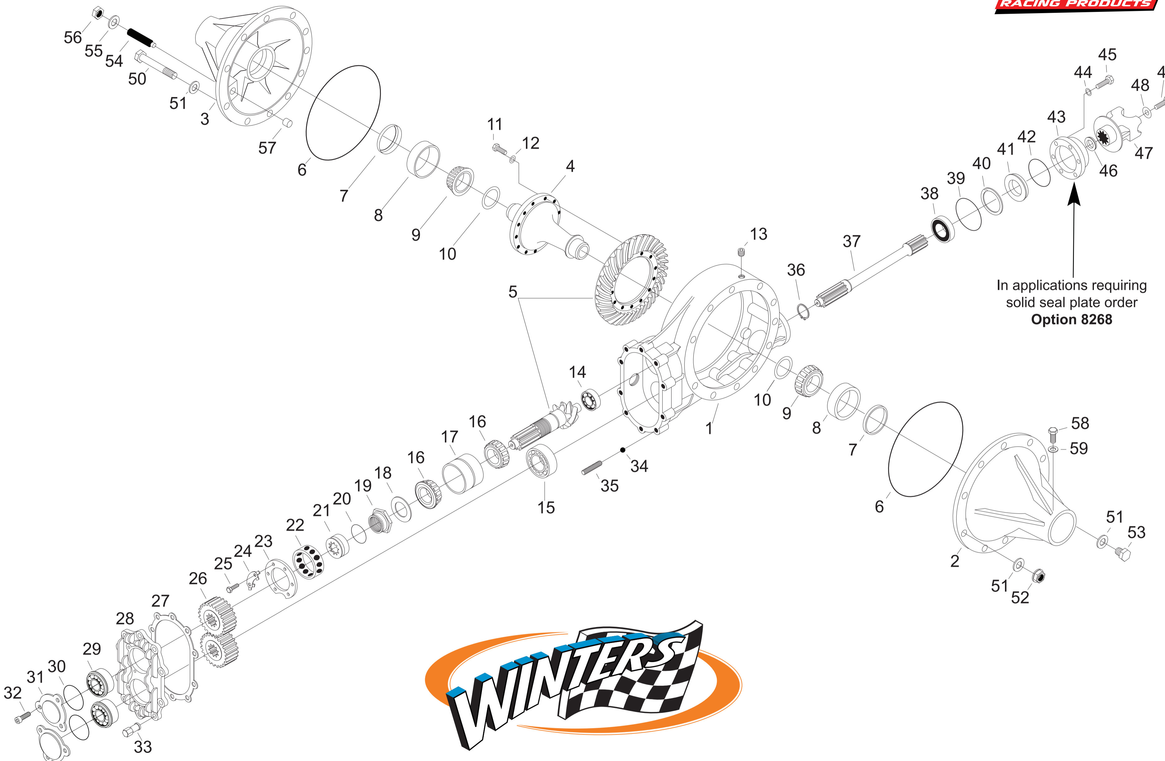
Winters 10" Rear End Exploded View
