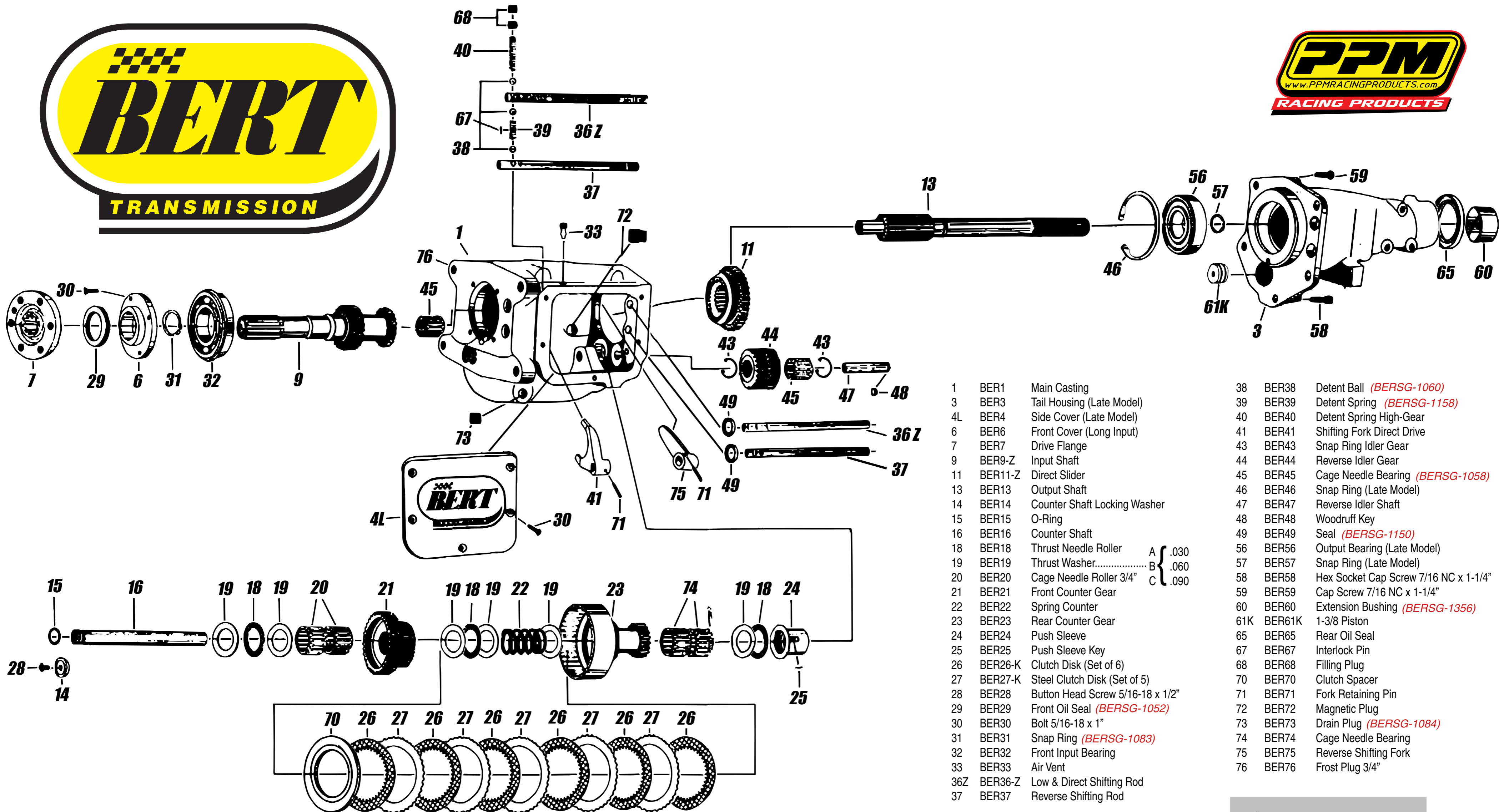
Bert 1st Generation Exploded View
